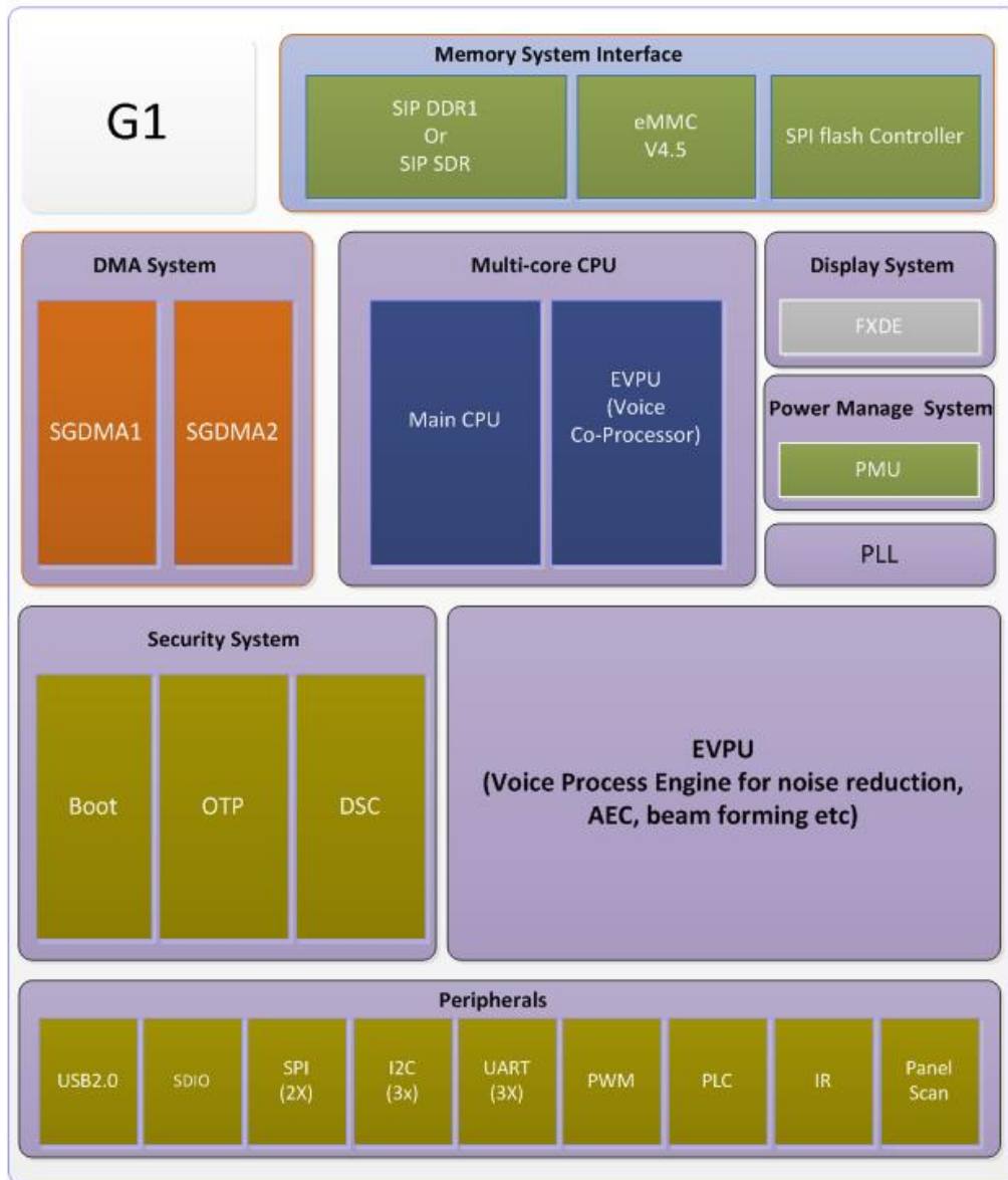
G1 architecture diagram with Audio Codec
